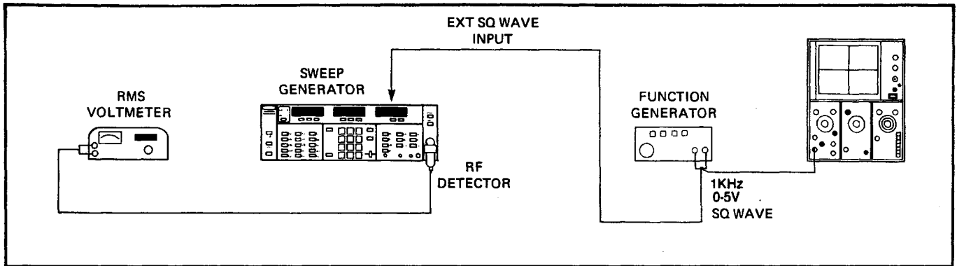
Figure 4-8. Test Equipment Setup for Residual AM Test
