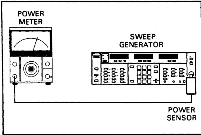
Figure 5-39. Test Equipment Setup for RF SLOPE and Power Level Adjustments
