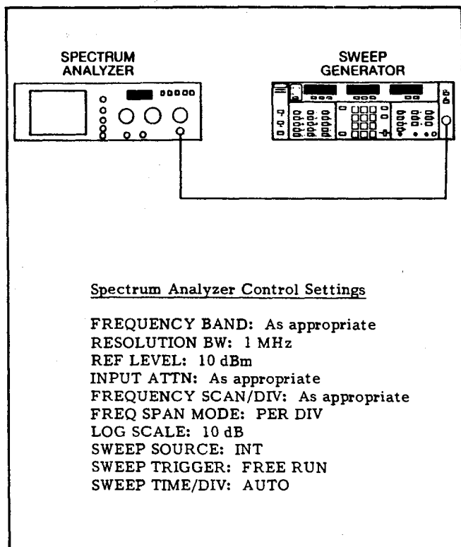
Figure 4-15. Test Equipment Setup for RF Output Signal Tests
