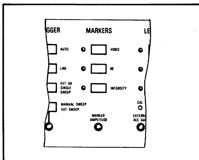
Figure 3-15. MARKERS Pushbuttons
