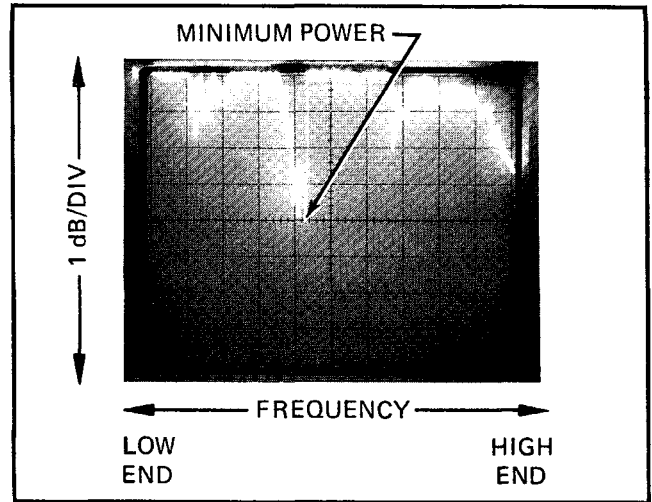
Figure 4-6. Unleveled Power
