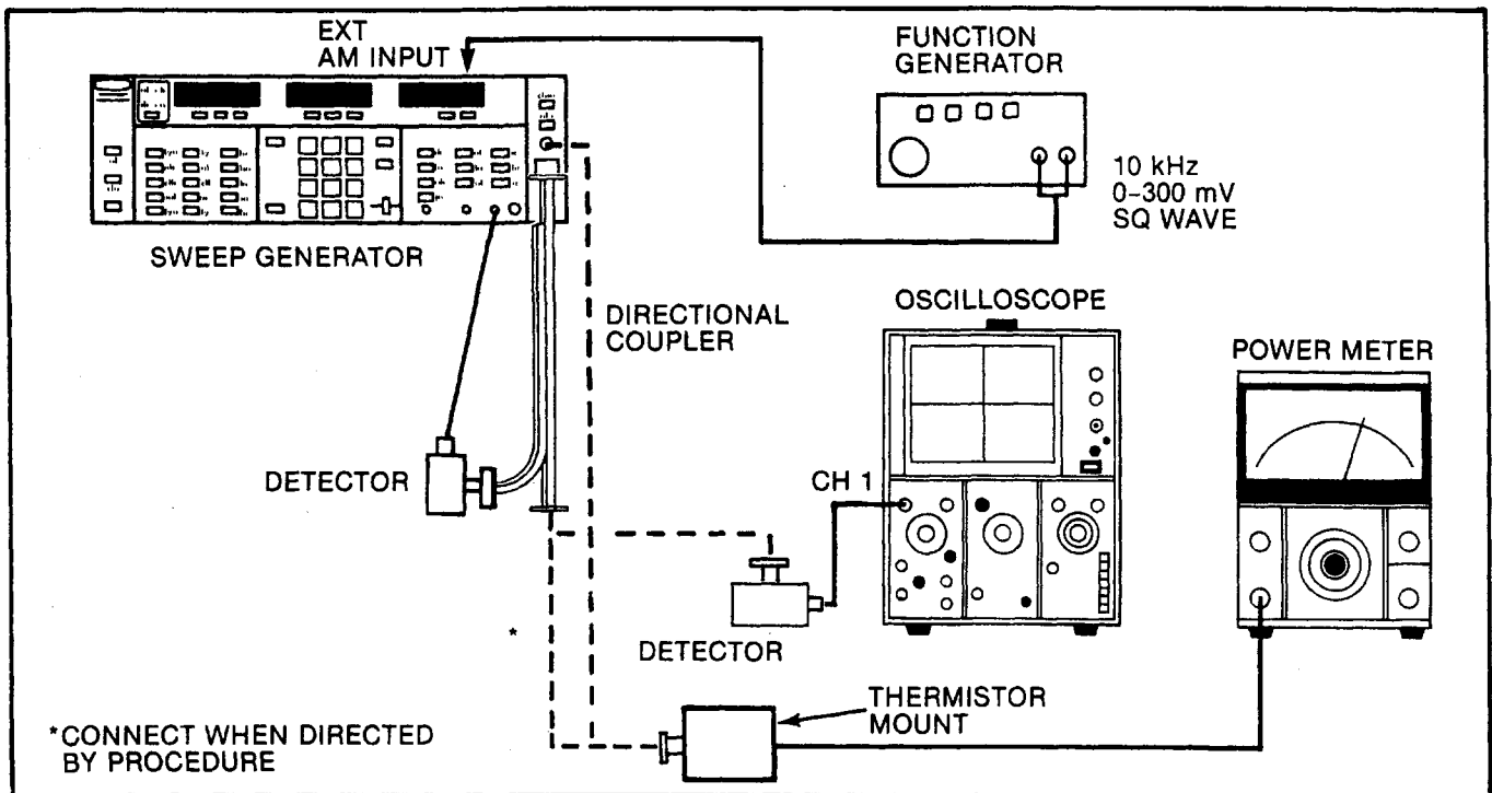
Figure 5-42. Model 6642A, Test Equipment Setup for Making ALC Loop Calibration Adjustments
