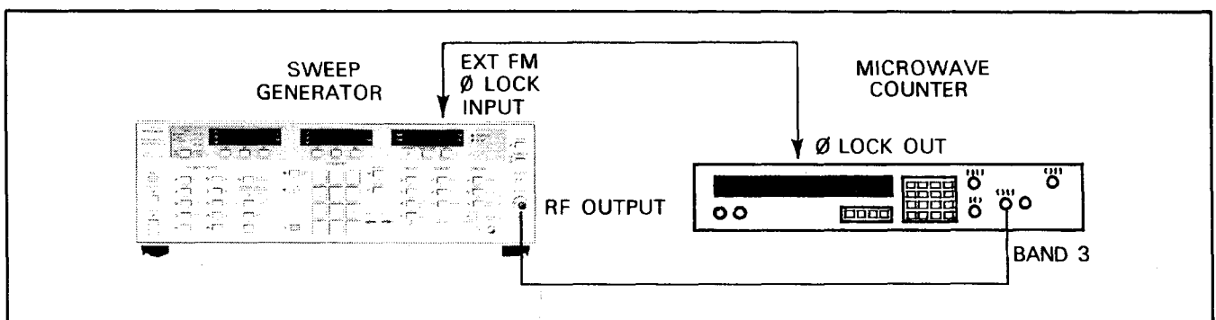
Figure 3-24. Test Setup for Operational Checkout of FREQUENCY VERNIER Controls (All models except 6642A)
