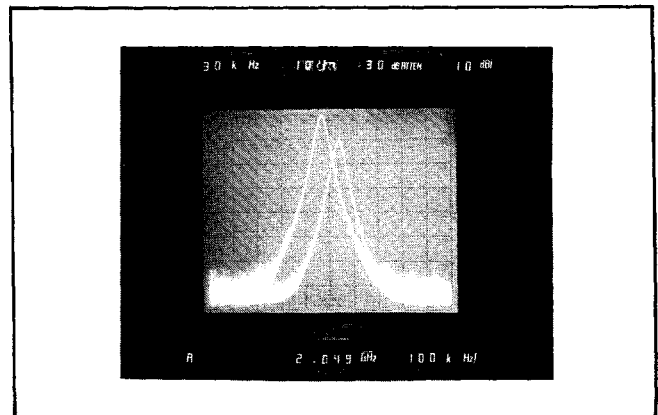
Figure 4-27. Example of Frequency Pulling
