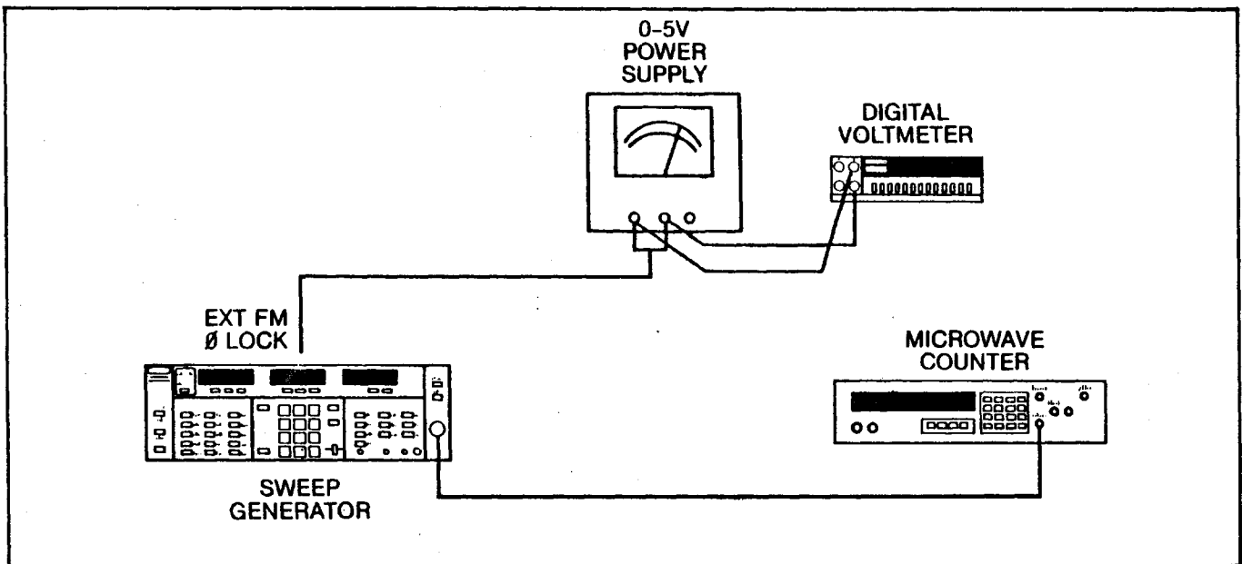
Figure 4-14. Test Equipment Setup for FM Deviation Test
