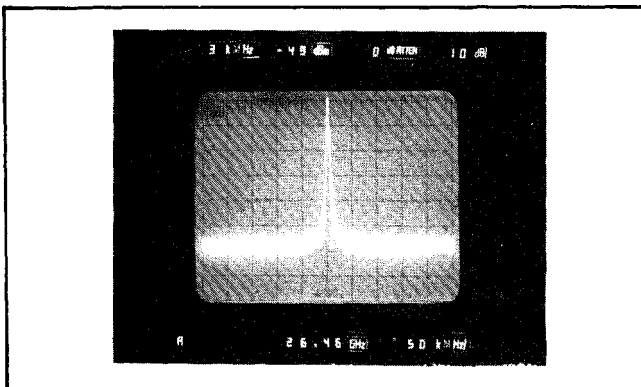
Figure 4-20. Analyzer Display, with 30 dB Signal-to-Noise Ratio
