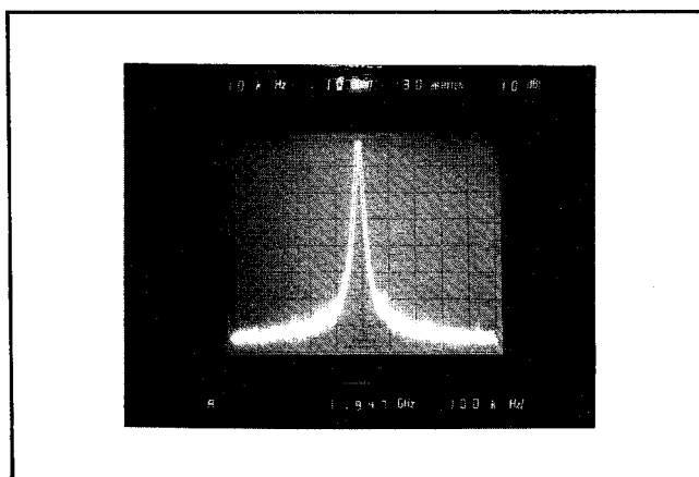
Figure 4-17. Noise Sidebands
