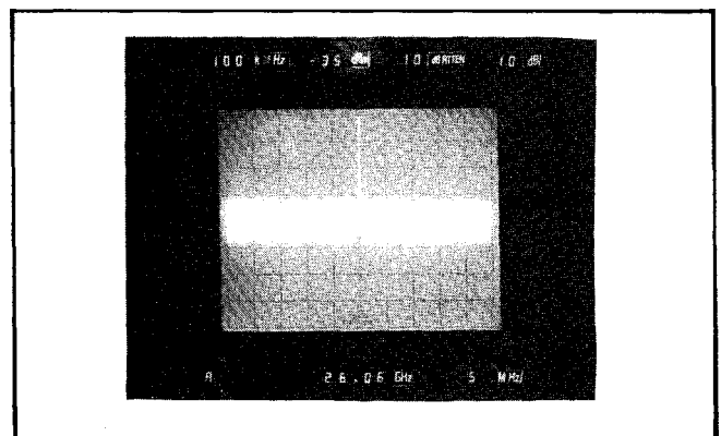
Figure 4-24. Analyzer Display, With 30 dB Signal-To-Noise Ratio
