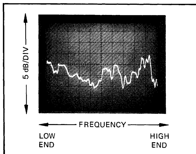
Figure 4-7. Leveled Power
