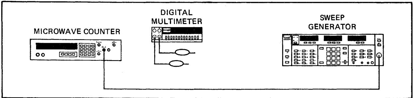
Figure 5-23. Test Equipment Setup for Frequency Calibration
