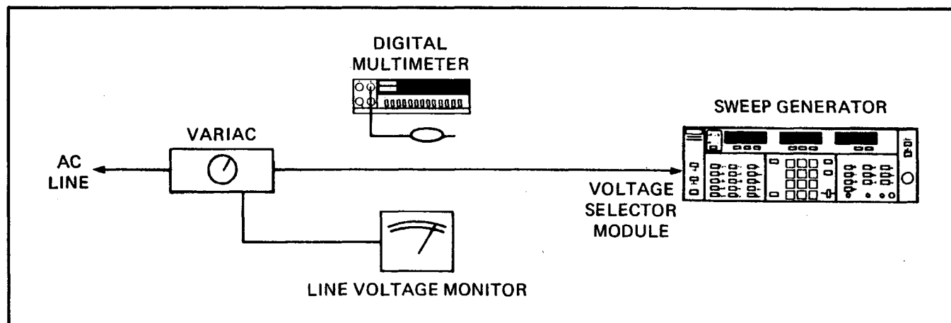
Figure 5-1. Test Equipment Setup for Low- and High-Line Adjustments
