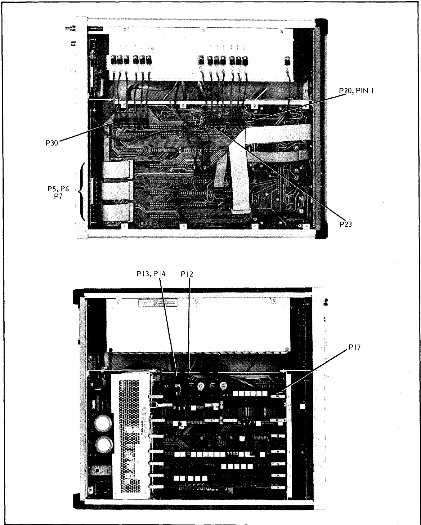
Figure 5-2. Connector Locations
