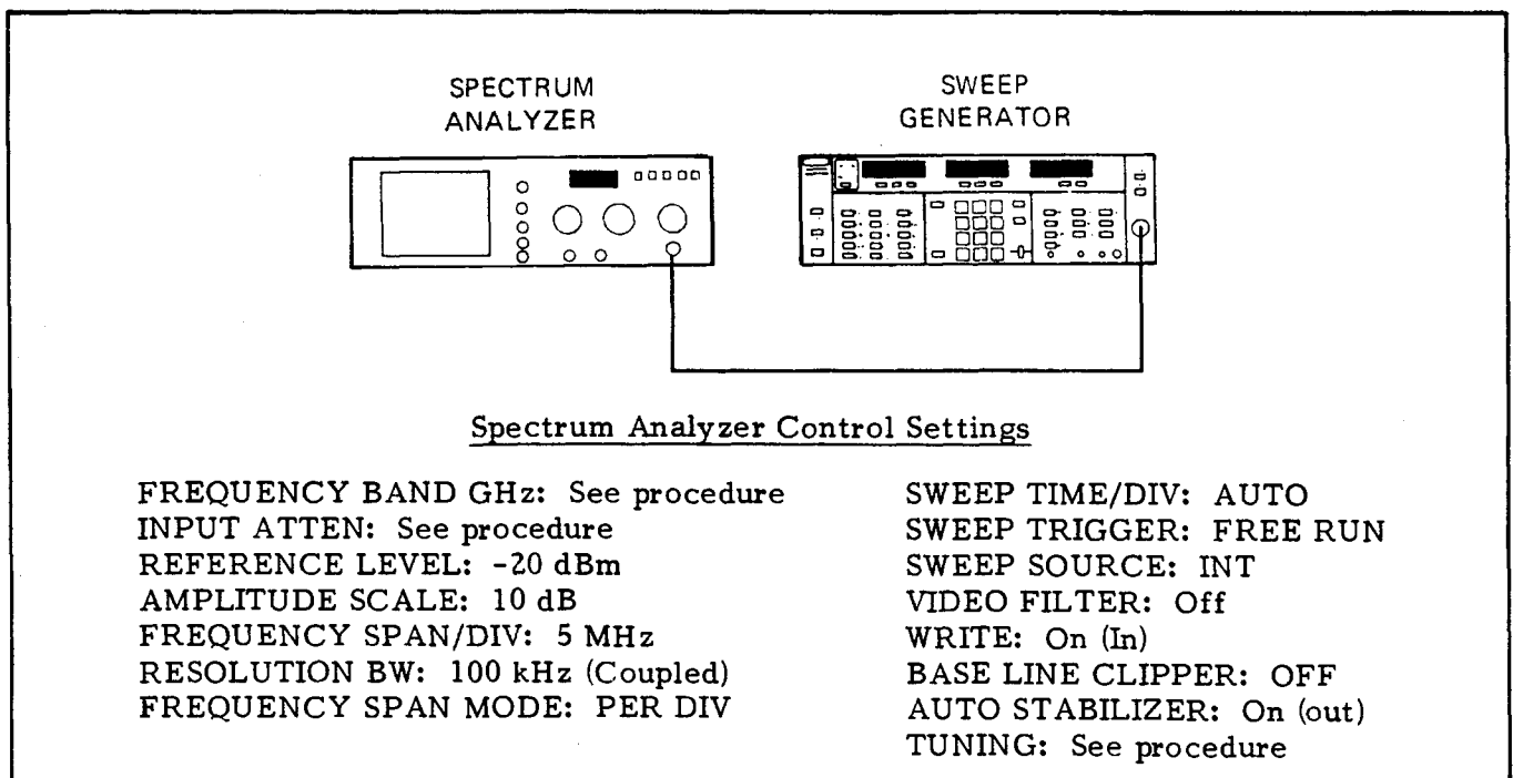
Figure 5-10. Test Equipment Setup For Frequency-Band Overlap Test
